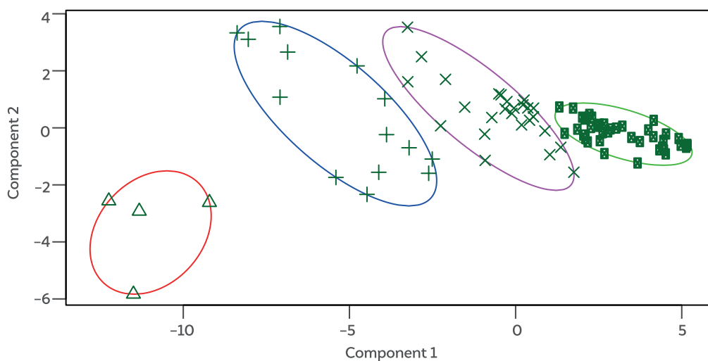
Figure A.9 Cluster plot against first two principal components for the household load profile for the month of September
