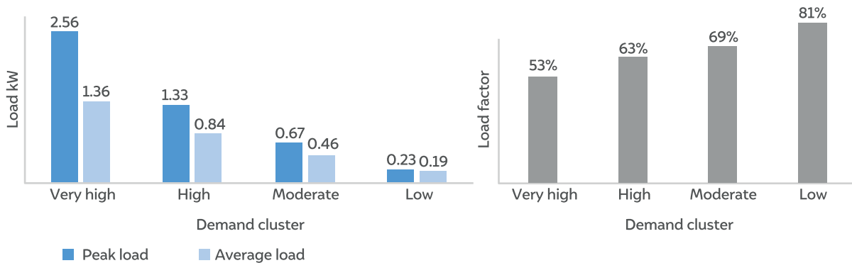
Figure 15: The load factor of households in very high demand clusters is less than 60 per cent
